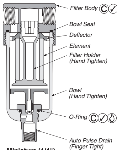
Miniature (1/4") Particulate Filter
