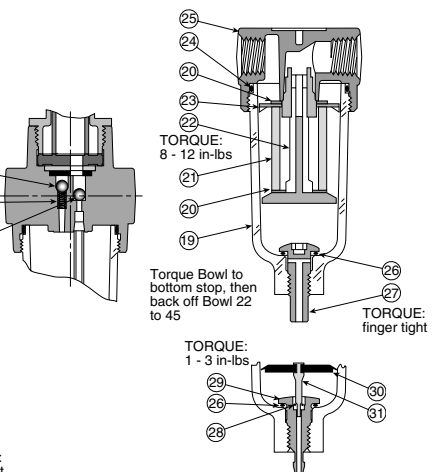
Figure 2: Particulate Filter
