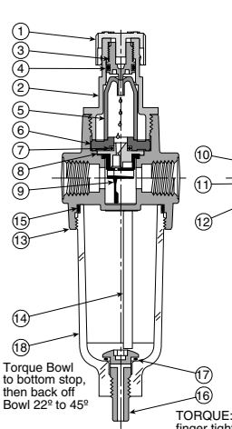
Figure 1: Mist Lubricator
